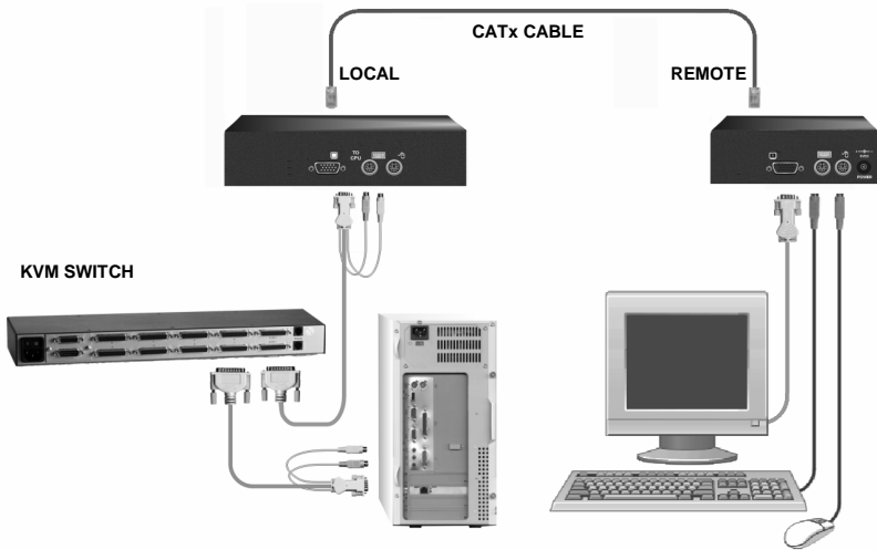
Figure 9. CrystalView Plus to a KVM switch
