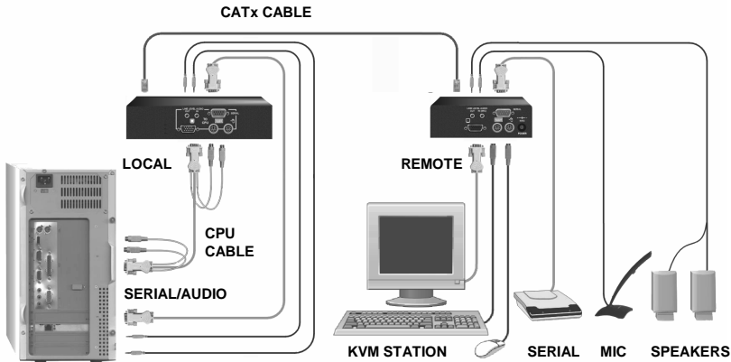
Figure 6. Single video cabling
