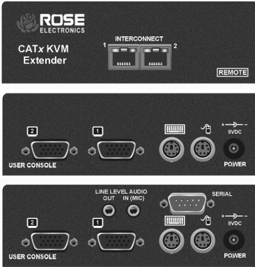
Figure 4. Dual video (Remote models)
