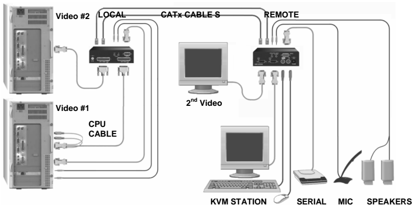
Figure 7. Dual video cabling
