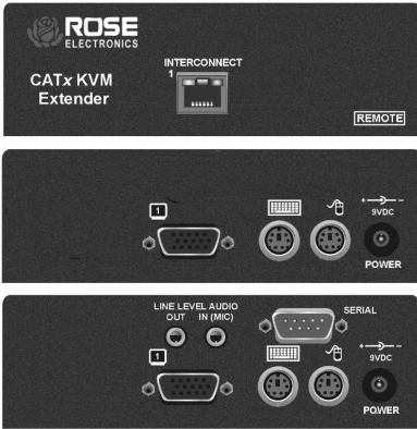
Figure 2. single Video (Remote models)
