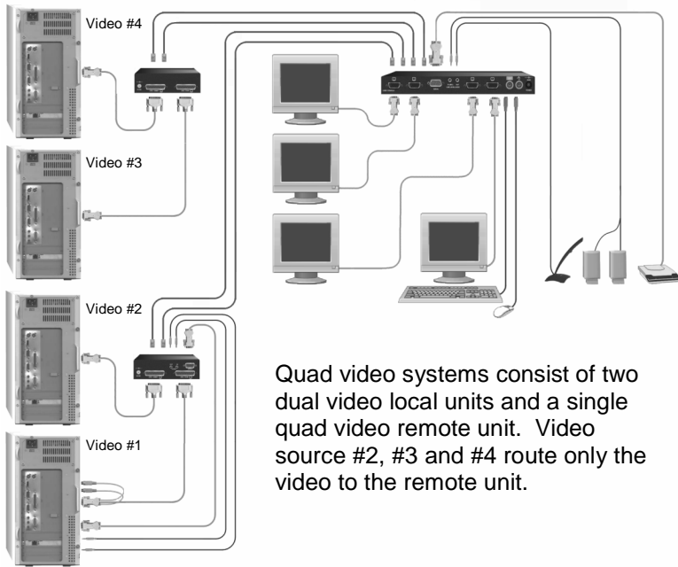
Figure 8. Quad video cabling
