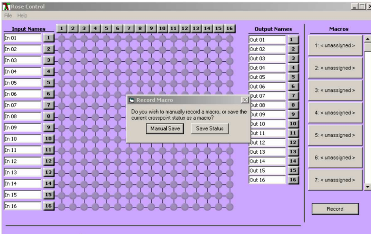
Figure 8. Macros
