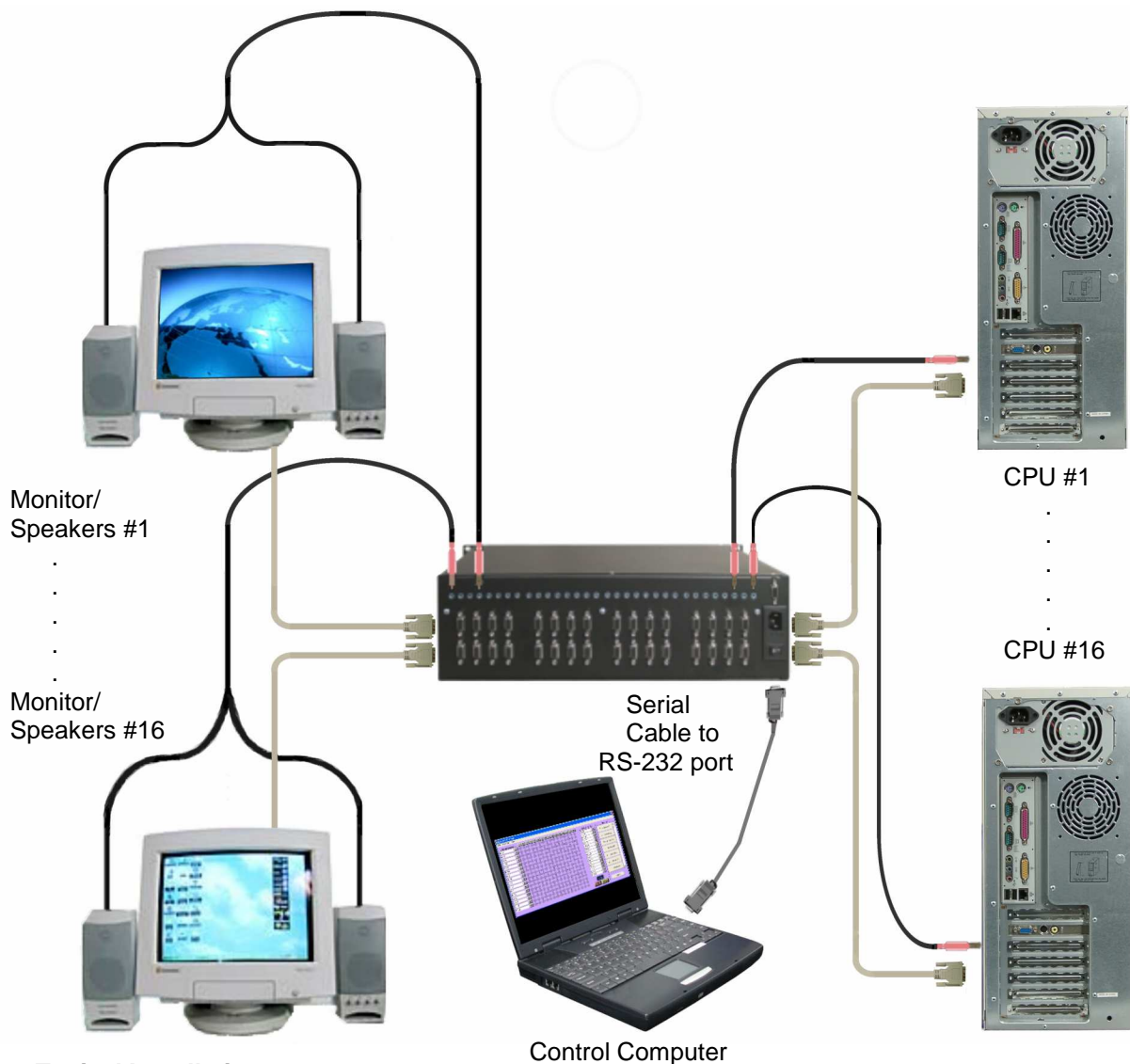
Figure 1. Typical Installation
