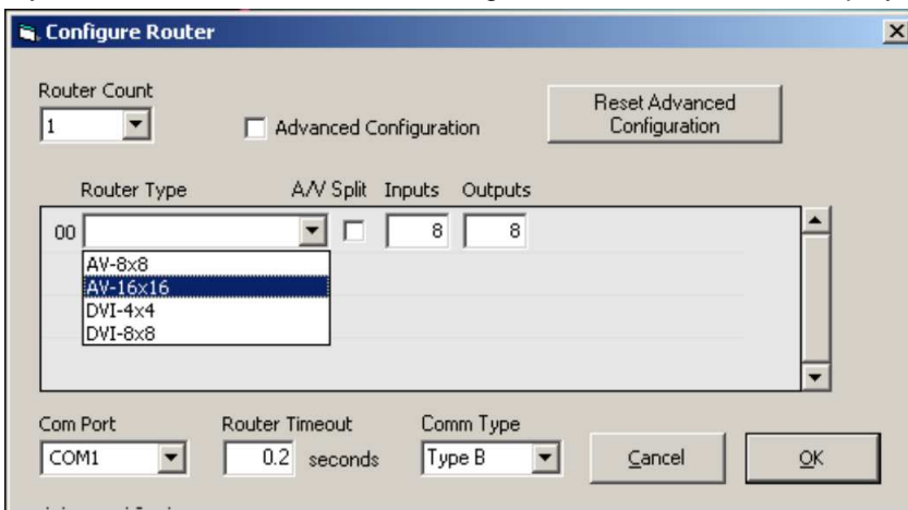
Figure 2. Configure Router
